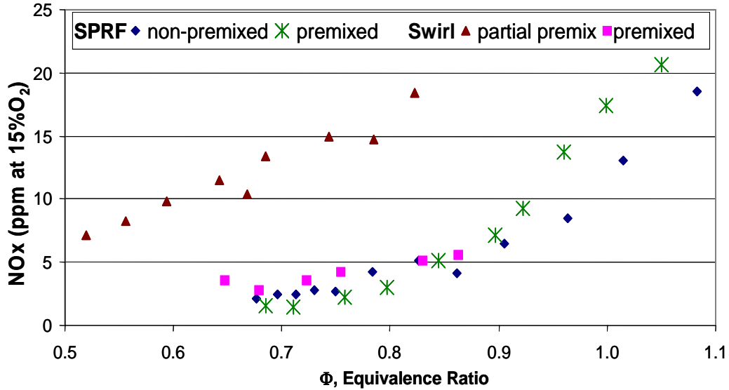
Figure 4. Dependence of NOx emissions on the global equivalence ratio of injected reactants.
